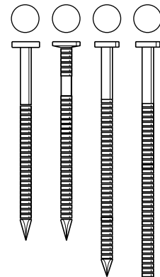
.099", .113", .120" 2" - 3"
